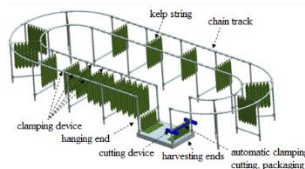
Figure 1: Double Track Drying Mechanism
