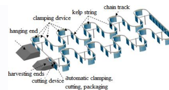
Figure 2: Single Track Drying Mechanism
